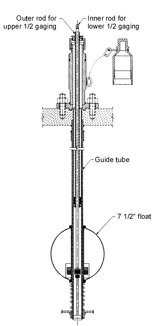
TANK EMPTY
